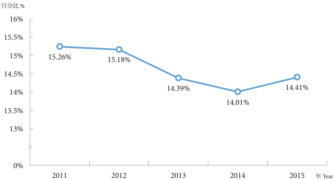
近五年首次捐血比率趨勢圖 Trends in the Rate of First-time Donors, 2011-2015
