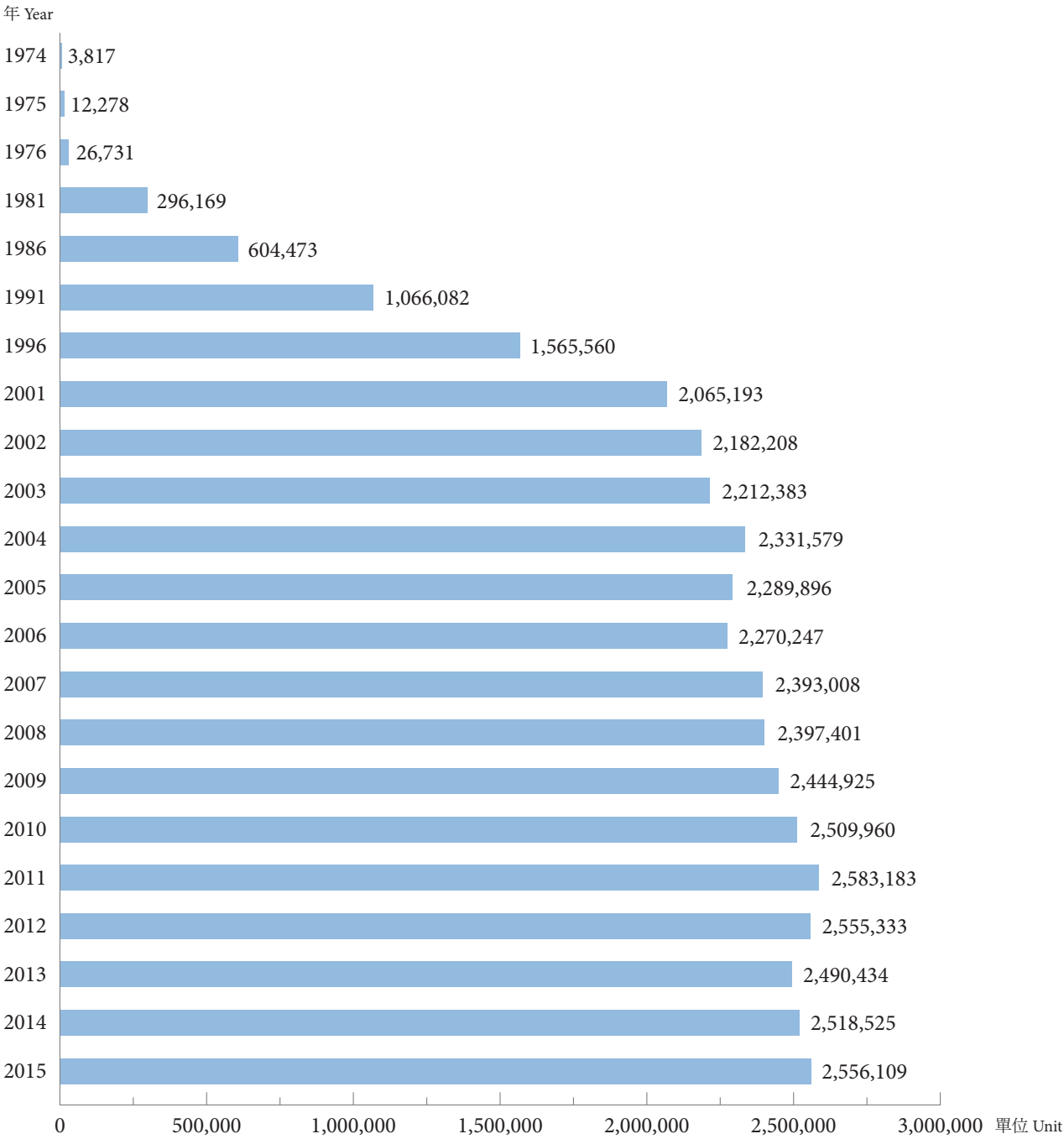
歷年捐血量趨勢圖 Annual Blood Collection, 1974-2015
