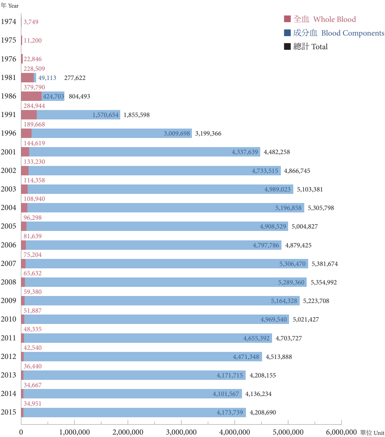
歷年供血量趨勢圖 Annual Blood Supply, 1974-2015
